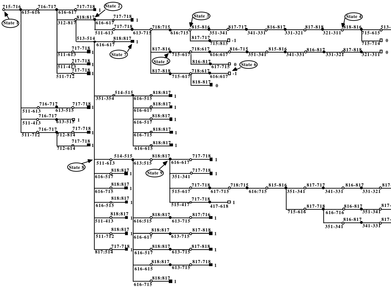
Fig. 4. Search tree for the optimization problem for space vehicles within the horizon 4.
