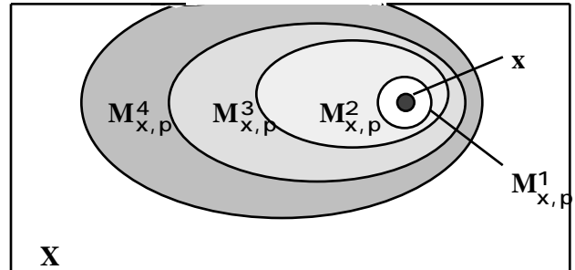
Fig. 1. Interpretation of the family of reachability areas Let MAP_{x,p}(y)=k , for y from M^k_{x,p} (the number of steps from x to y ). For the remaining points, let MAP_{x,p}(y)=2n , if y \notin X ( n is the number of points in X ); MAP_{x,p}(y)=0 , if y = x .
